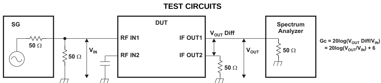
Figure 18. Conversion Gain-Measurement Circuit
