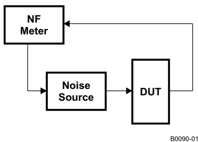
Figure 19. Noise-Figure Measurement Circuit
